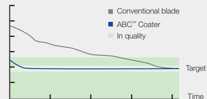
Chart showing the 2-Sigma value over time. The first 2-Sigma value from the scanner is normally twice as good compared to a conventional system.
