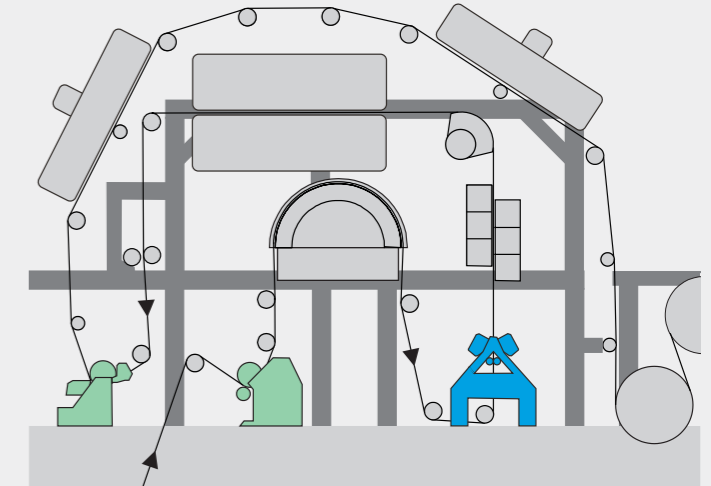
Future: 2+2 coating layers within the same machine space
